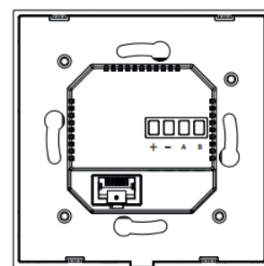
4 BACK VIEW
