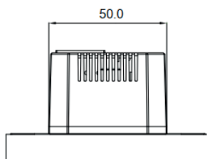
6 TOP VIEW
