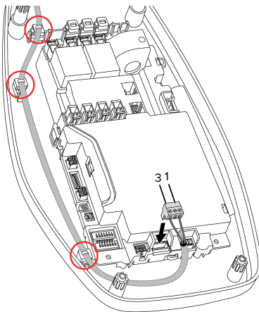
Fig. 9: Shunt release connection
