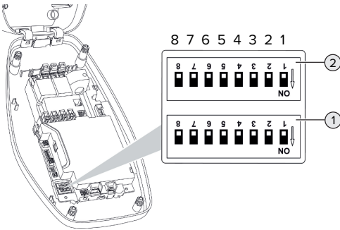
Fig. 11: DIP switches (delivery state)
