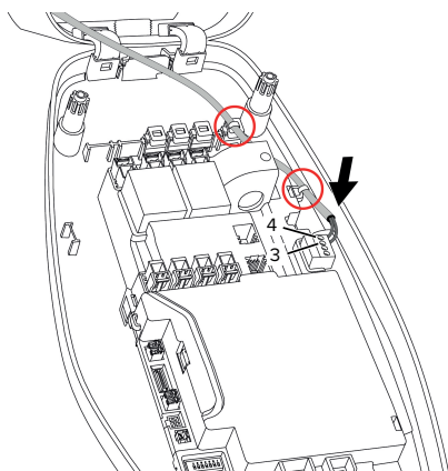
Fig. 12: Tilkobling Downgrade-inngang
