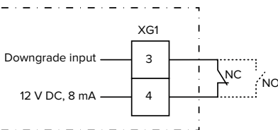
Fig. 13: Schematic circuit diagram: Connection of an external switching contact (default setting: NO)
