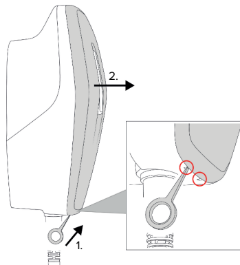
Fig. 4: Soltar o painel frontal
