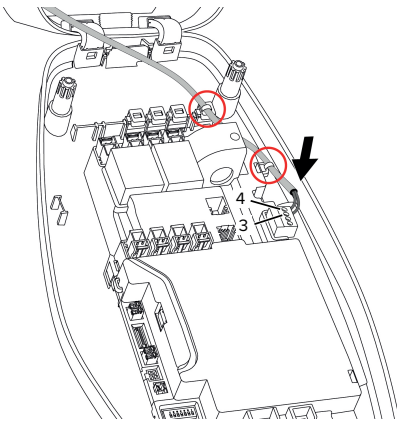
Fig. 12: Downgrade input connection
