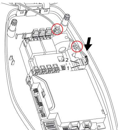
Fig. 14: Enable input connection
