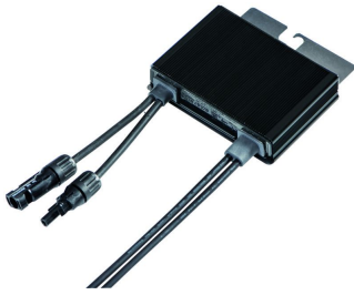
SolarEdge Optimierer 500W/60V/15A Kabel 2,3m OUT/0,1m IN
