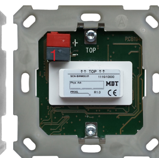
SCN-BWM55xxx.x2 Back
